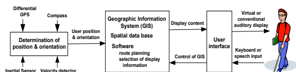
Fig. 1. Functional block diagram of the navigation system proposed by Loomis et al, adapted from [2].
