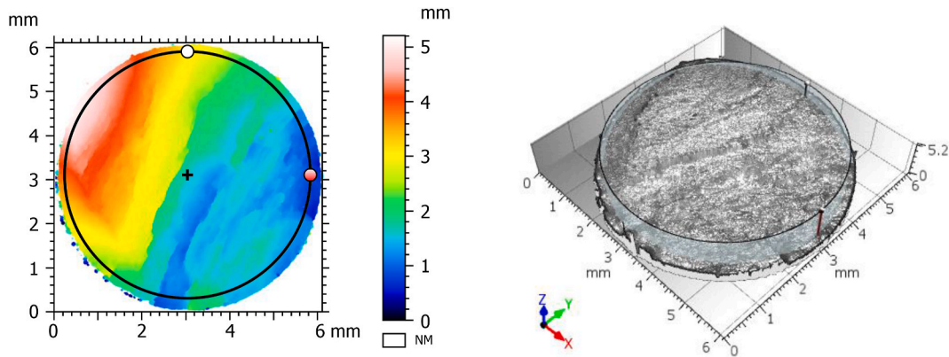
Fig. 3. Original and marked final surfaces in pseudo-color and grey views for specimen 15 (side B). (For interpretation of the references to color in this figure legend, the reader is referred to the Web version of this article.)
