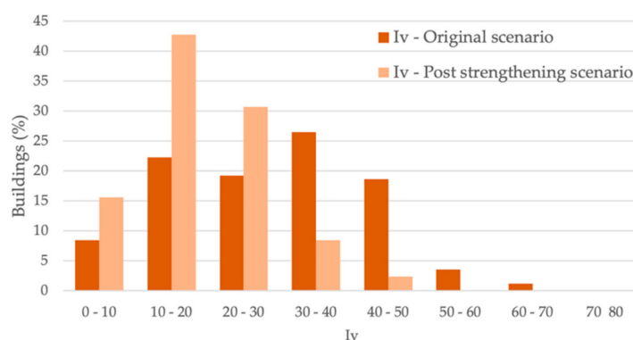
Figure 10. Comparison of the vulnerability index pre- and post-strengthening.
