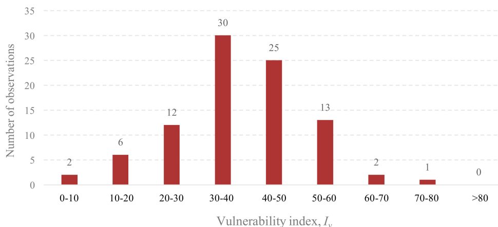
Figure 3. Distribution of the analyzed buildings over ranges of vulnerability index values.
