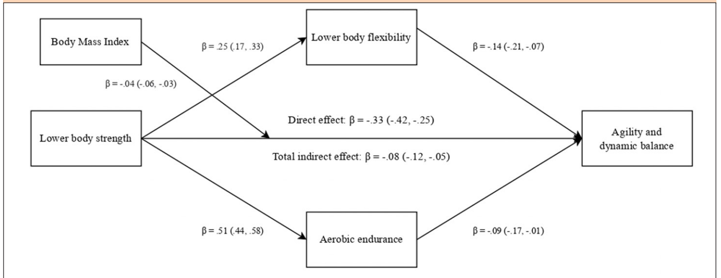
Figure 1. Mediated-moderation model
