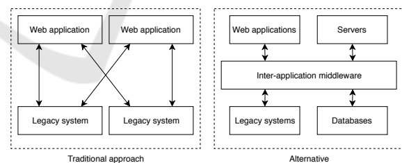
Figure 1: Comparison of two software architectural approaches for EAI.
