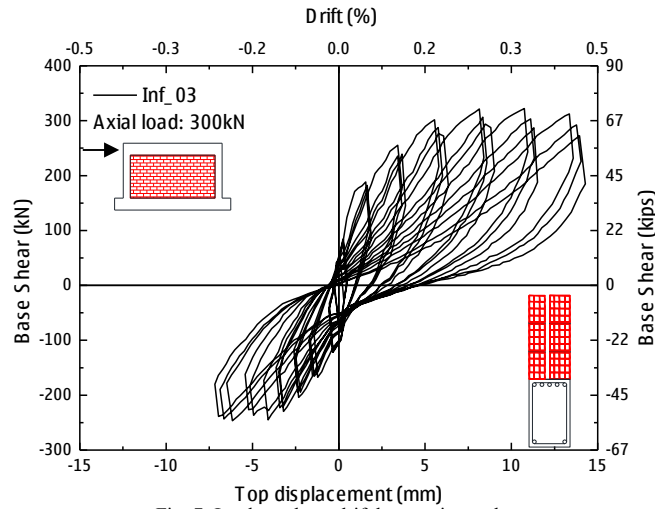
Fig. 7: In-plane shear-drift hysteretic results
