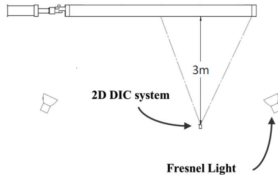
Fig. 6: Digital Image correlation setup.
