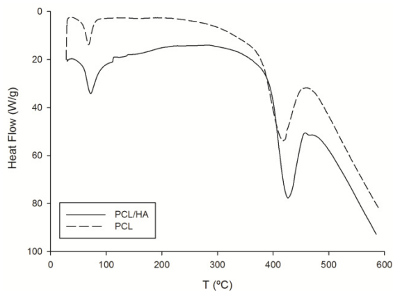
Fig. 3. Thermal curves of the scaffolds.
