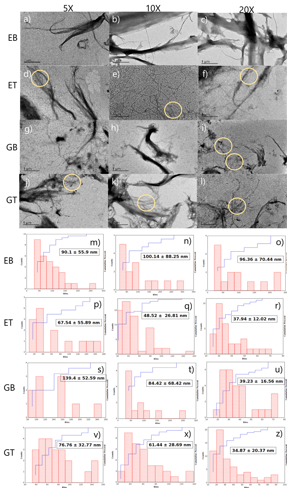
Fig. 1. Micrographs of the EB, ET, GB and GT suspensions with different steps: a) EB 5 steps, b) EB 10 steps, c) EB 20 steps, d) ET 5 steps, e) ET 10 steps, f) ET 20 steps, g) GB 5 steps, h) GB 10 steps, i) GB 20 steps, j) GT 5 steps, k) GT 10 steps and l) GT 20 steps. All images are at 5000× magnification and with 1 μm scale. Measurements of fiber sizes in treatments m) EB 5 steps, n) EB 10 steps, o) EB 20 steps, p) ET 5 steps, q) ET 10 steps, r) ET 20 steps, s) GB 5 steps, t) GB 10 steps, u) GB 20 steps, v) GT 5 steps, x) GT 10 steps and z) GT 20 steps.
