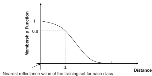
Figure 2: Membership function used in the fuzzy classifier based on the Nearest Neighbor Classifier.
