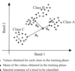
Figure 1: Nearest Neighbor Classifier.
