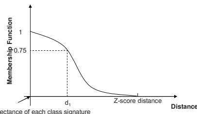
Figure 4: Membership function used in the fuzzy classifier based on the Minimum-Distance-to-Means Classifier
