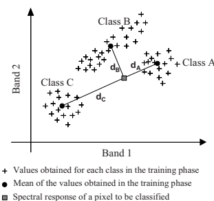
Figure 3: Minimum-Distance-to-Means Classifier.
