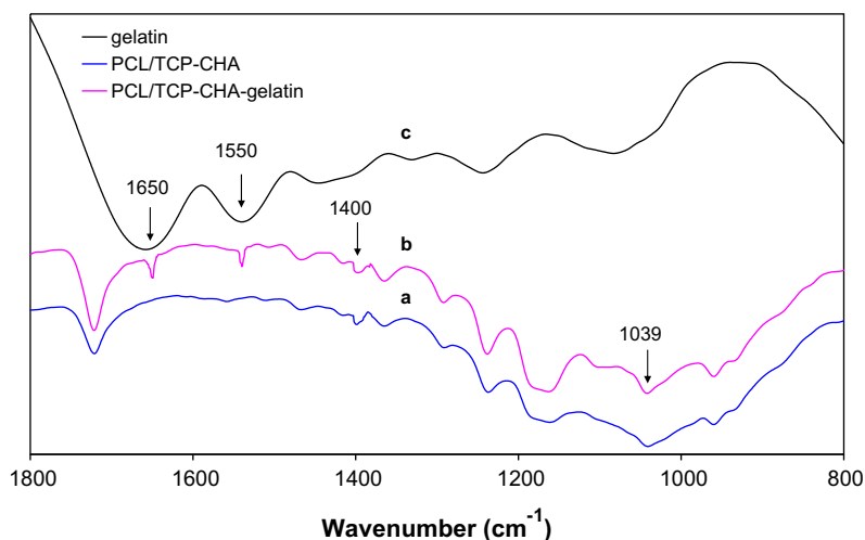
Fig. 3. ATR-FT-IR spectra of (a) PCL/TCP, (b) PCL/TCP-CHA, and (c) PCL/TCP-CHA-gelatin scaffolds.
