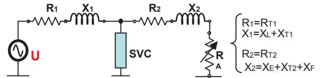
Figure 5. Electrical equivalent circuit of the total system, where R_A is represented by Figure 3 and the resistances and reactances are the same as those of Figure 2.
