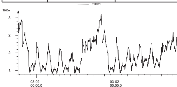
Figure 9. Chart of Total Voltage Harmonic Distortion of Phase 1 with SVC; arc furnace working at about 30 MW.
