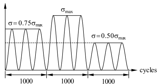
Fig. 2. Block load spectrum of the variable-amplitude high-cycle fatigue test program.
