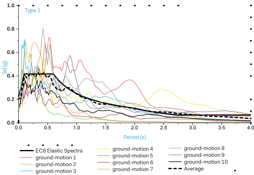
Figure 32 - Elastic spectrum of the ground motions selected (Type 1)
