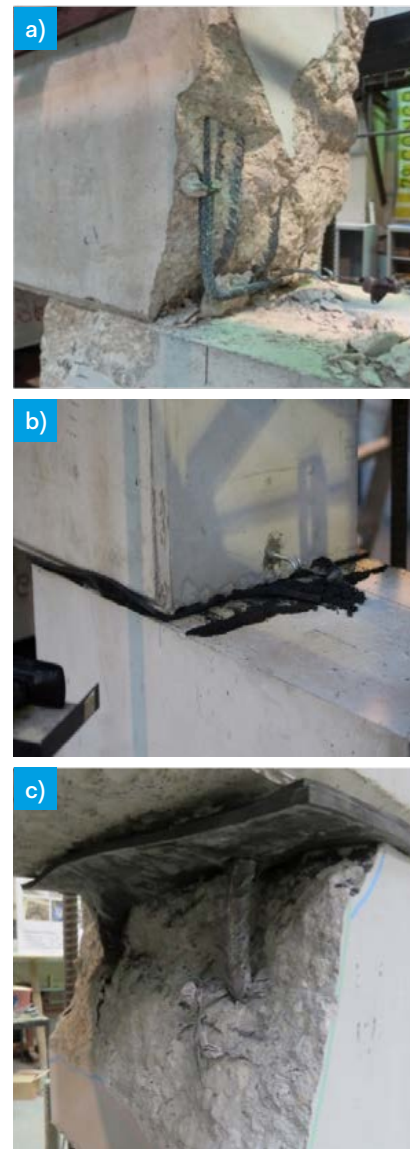
Figure 25 · Damages observed in the specimens
