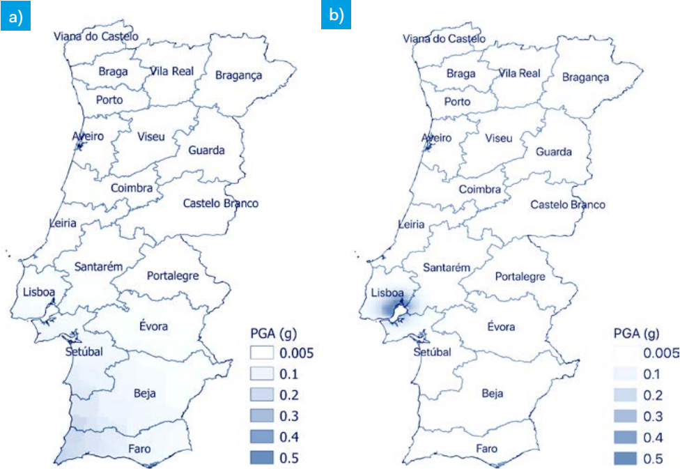
Figure 44 · Mean ground motion fields for a) the offshore and b) onshore scenario
