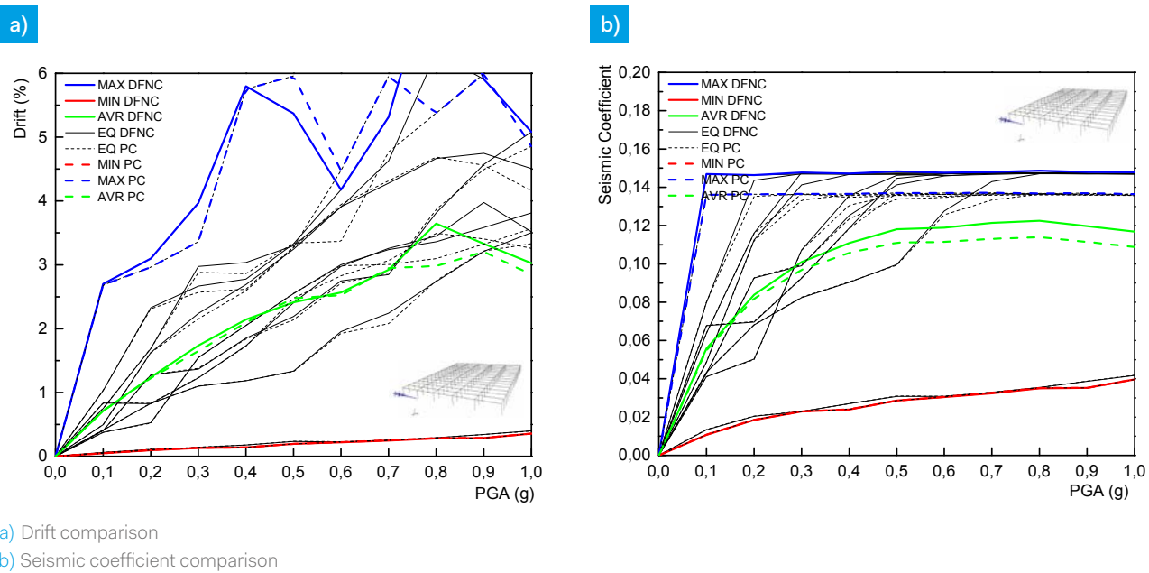
Figure 33 · Model 3D with pinned and DFNC connections for earthquake type 1 in X direction
