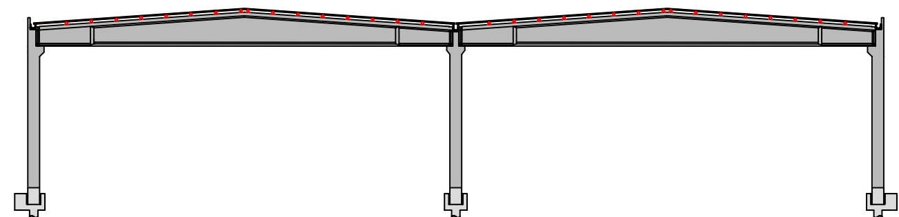
Figure 13 · Illustration of the main PRC typologies identified in Portugal with a variable cross-section I shaped prestressed beams
