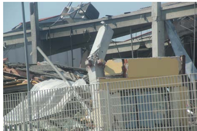
Figure 2 - Short-column effect due to the interaction with irregular masonry walls
