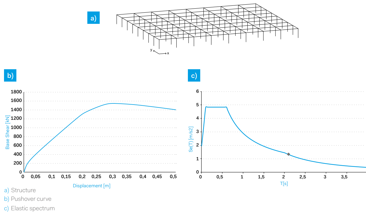
Figure 38 - Input data to N2 method
