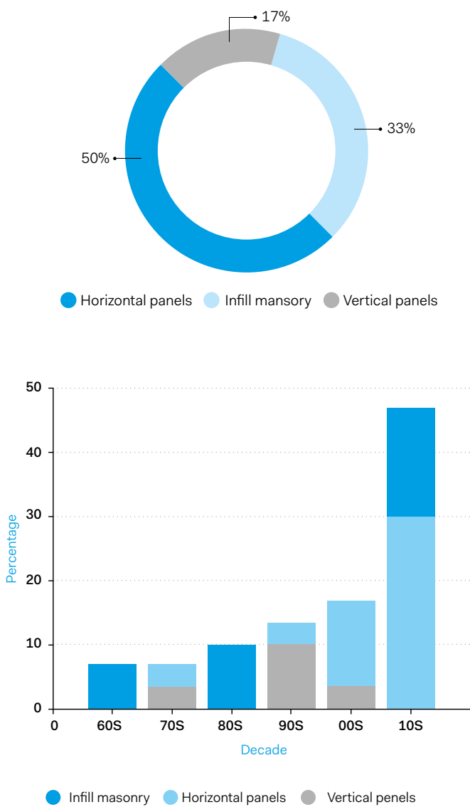
Figure 17 · Variation of type of cladding system by decade
