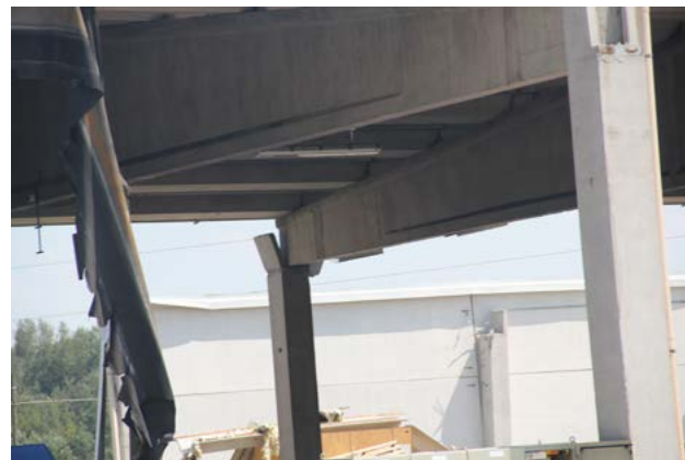
Figure 3 - Collapse of the forks at the top of the columns due to out-of-plane actions
