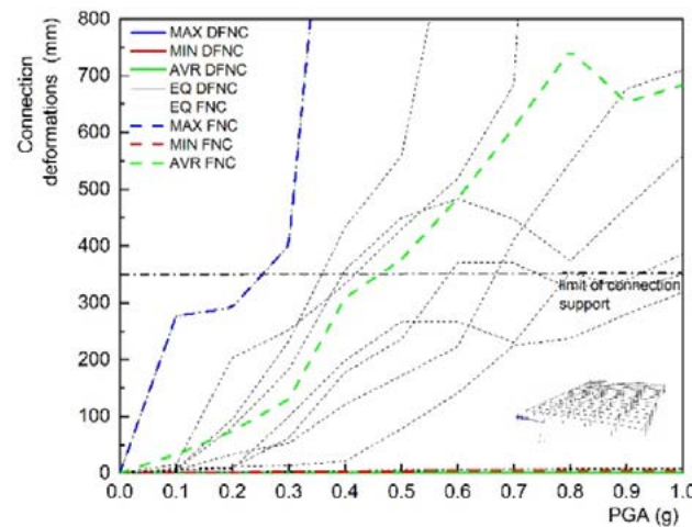
Figure 36 - Connection sliding in model 3D (12 m) with DFNC and FNC
