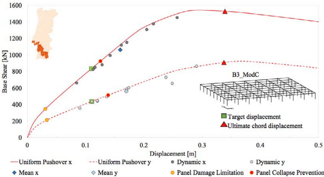
Figure 43 · Dynamic results for x and y direction for building B3_ModC
