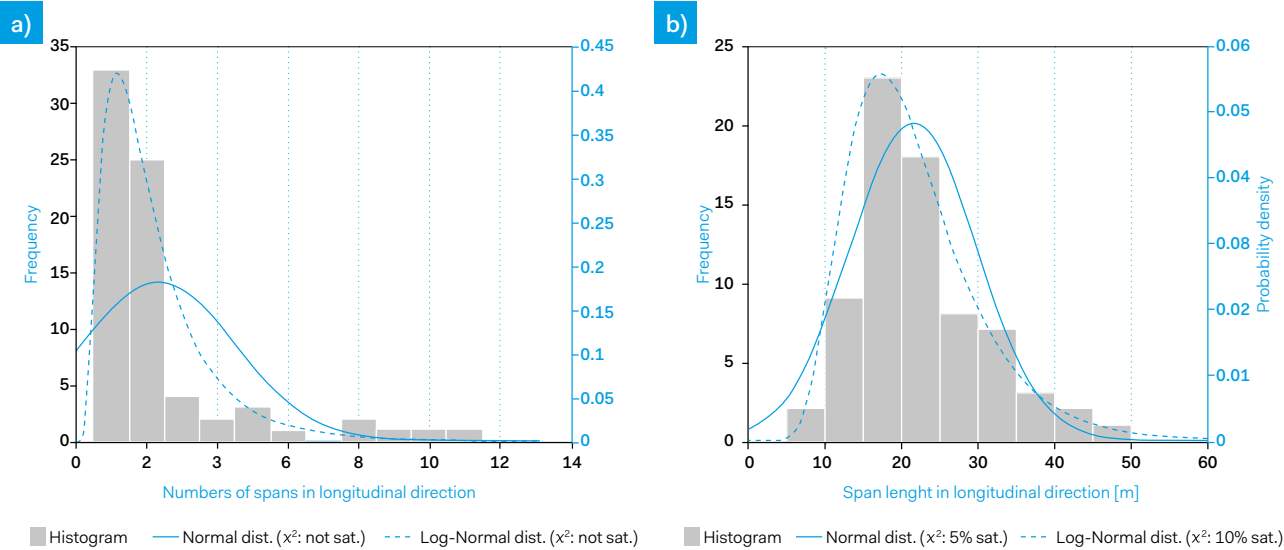
Figure 15 · Histogram and probability distributions associated with the: a) number and; b) length of the spans (in the longitudinal direction)
