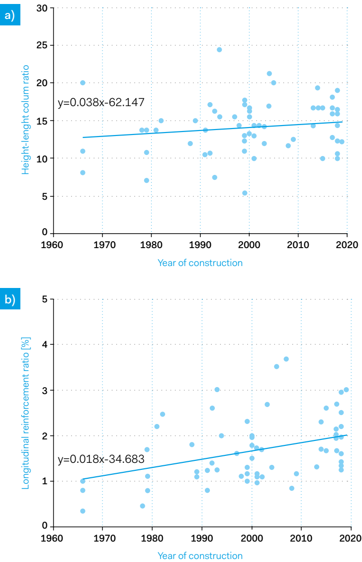
Figure 19 - a) Evolution of height-to-length column ratio and; b) Longitudinal reinforcement ratio with the year of construction
