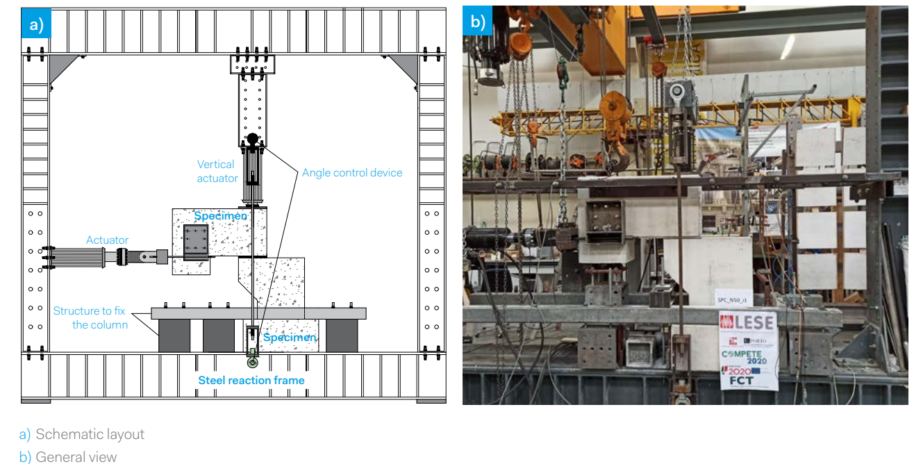
Figure 23 - Testing setup
