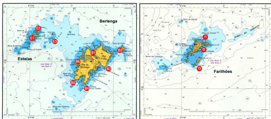
Figure 2. Location of the sampling stations in the 3 groups of islands of the Berlengas Natural Reserve
