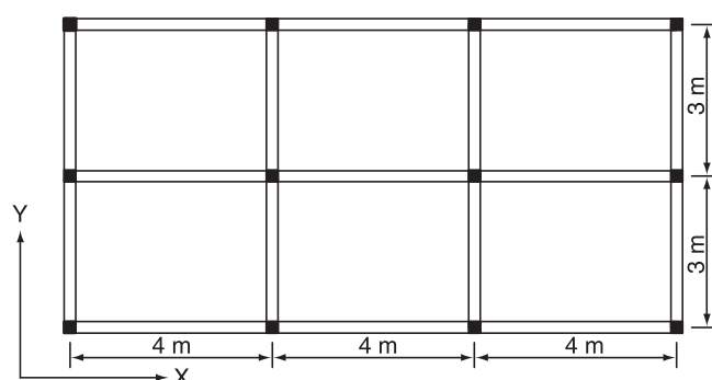
(a) Plan of the building
