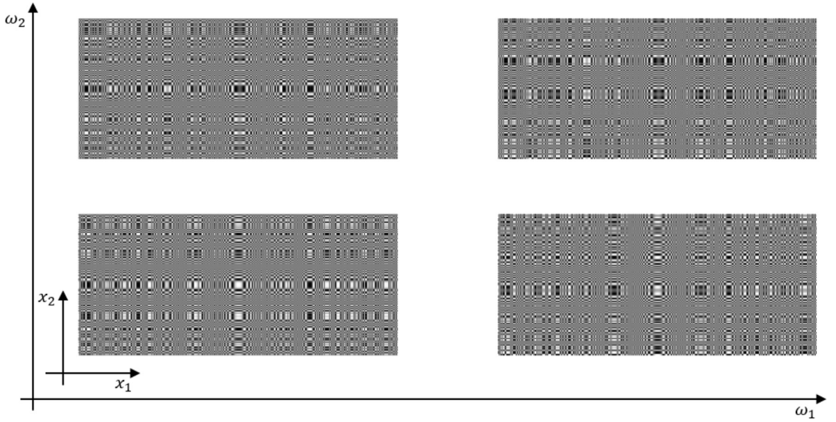
Fig. 1. The small images are intensity images of the basis function of the first component in (38), up to the dilation and phase factors 1/\sqrt{b_1}\mathbf{i} and 1/\sqrt{b_2}\mathbf{j} , with parameters t_1 = 20 and t_2 = 10 , A = (5, 3; 3, 2) , \omega_1 \in \{\pi/2, 2\pi\} , and \omega_2 \in \{\pi/4, 8\pi\} .
