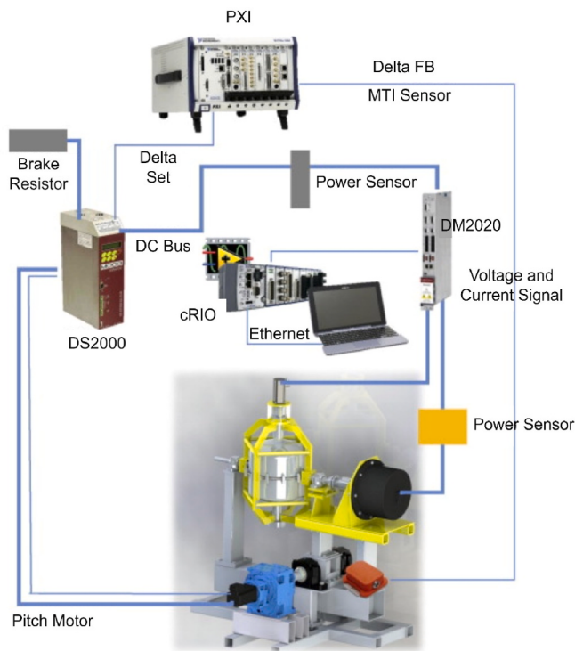
Fig. 12. ISWEC HIL setup. Legend: (DC) Direct Current, (FB) pitch angle feedback and (MTI) Inertial sensor. Adapted from Ref. [2].
