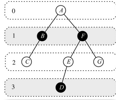
Fig. 3. Resulting BFS graph.
