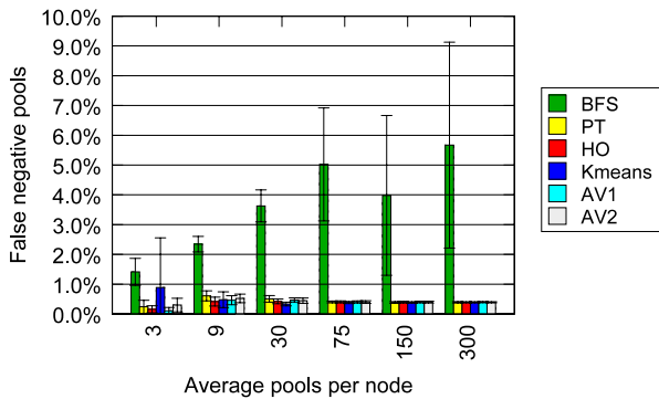
Fig. 9. False negatives for 20% of M_4 -type workers.
