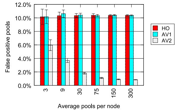
Fig. 12. Percentage of false positive pools in the whitewashing attack.
