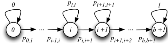
Fig. 2. Markov chain of the number of different correct nodes.
