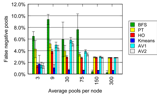
Fig. 7. False negatives for 20% of M_1 and 20% of M_2 .
