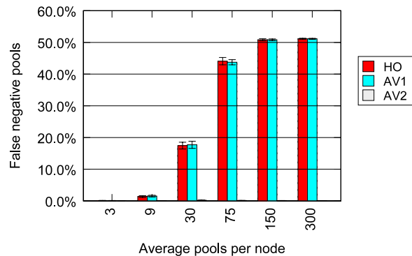
Fig. 13. Percentage of false negative pools in the whitewashing attack.
