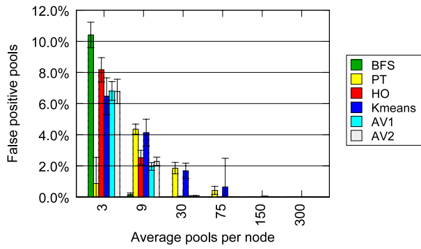
Fig. 4. Percentage of false positive pools for 20% of M_2 .
