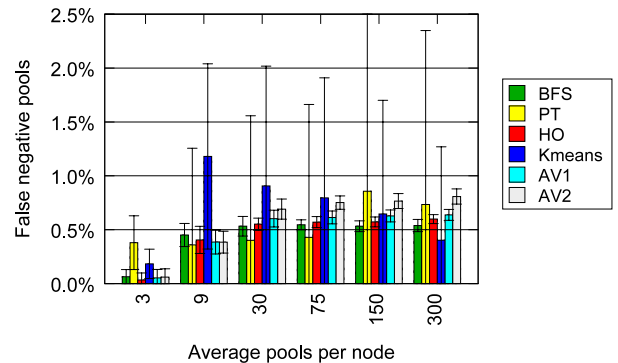
Fig. 11. False negatives for 20% of M_5 -type workers.
