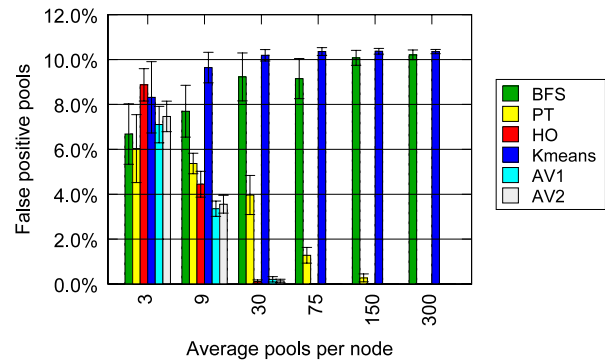
Fig. 6. False positives for 20% of M_1 and 20% of M_2 .
