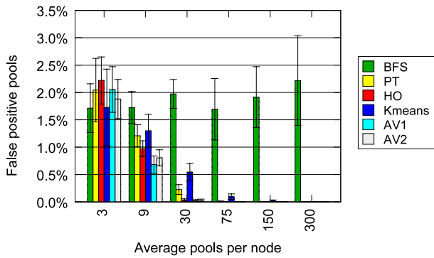
Fig. 8. False positives for 20% of M_4 -type workers.
