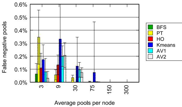
Fig. 5. Percentage of false negative pools for 20% of M_2 .
