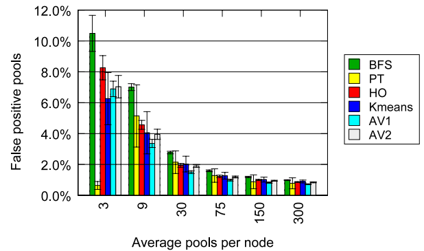
Fig. 10. False positives for 20% of M_5 -type workers.
