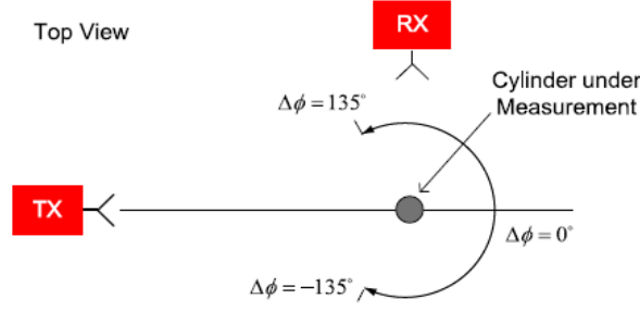
Fig. 1 – Measurement geometry.
