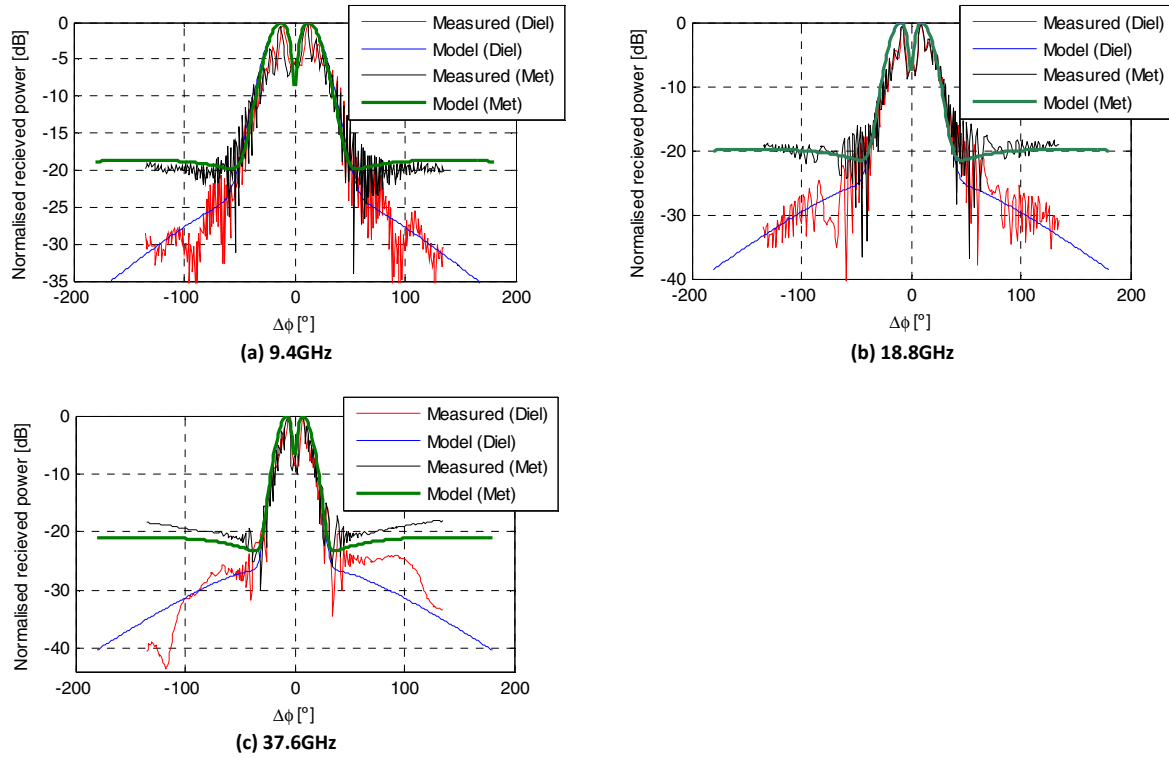
Fig. 2 – 37.6 GHz re-radiation measurement and model prediction comparison.
