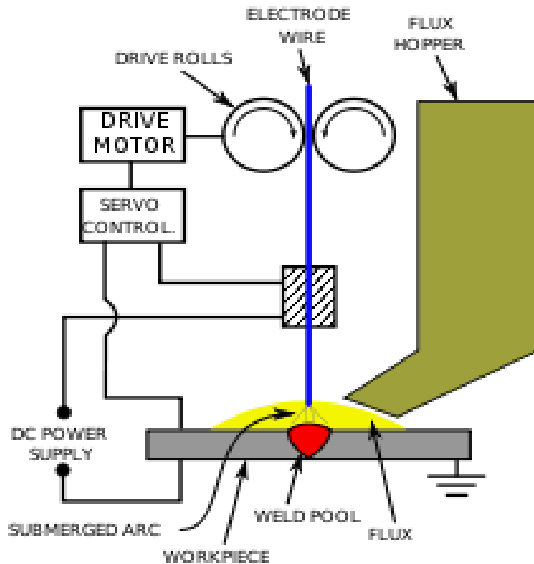
Figure 37: Submerged Arc Welding, process 121(Submerged Arc Welding)
