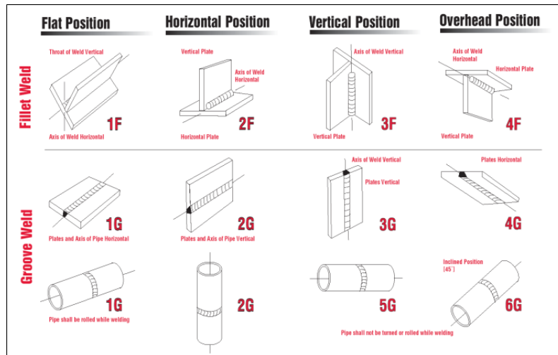
Figure 40: Various positions that a welding can be made (welding- Basic steps, terms, application, different welding joint and positions)
