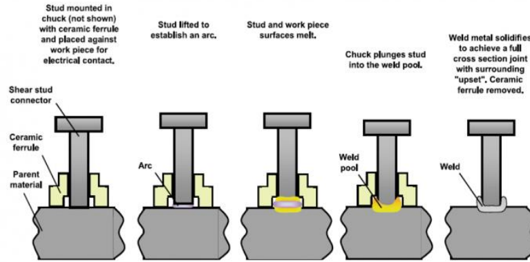
Figure 38: Drawn arc stud welding with ceramic ferrule, process 783(SteelConstruction.info- The free encyclopedia for UK steel construction information)
