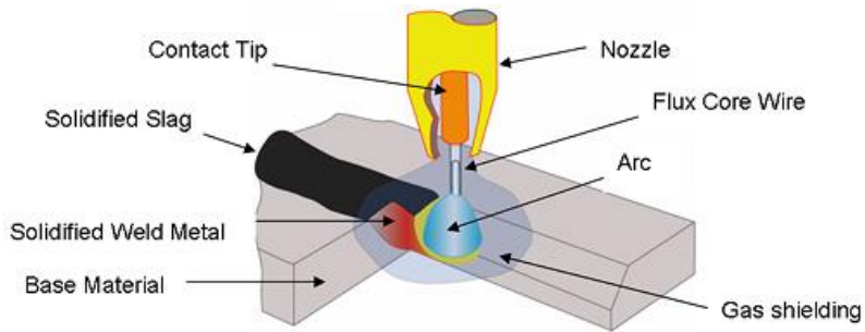
Figure 36: Flux Cored Arc Welding, process 136(Welding technology or techniques, 2016)
