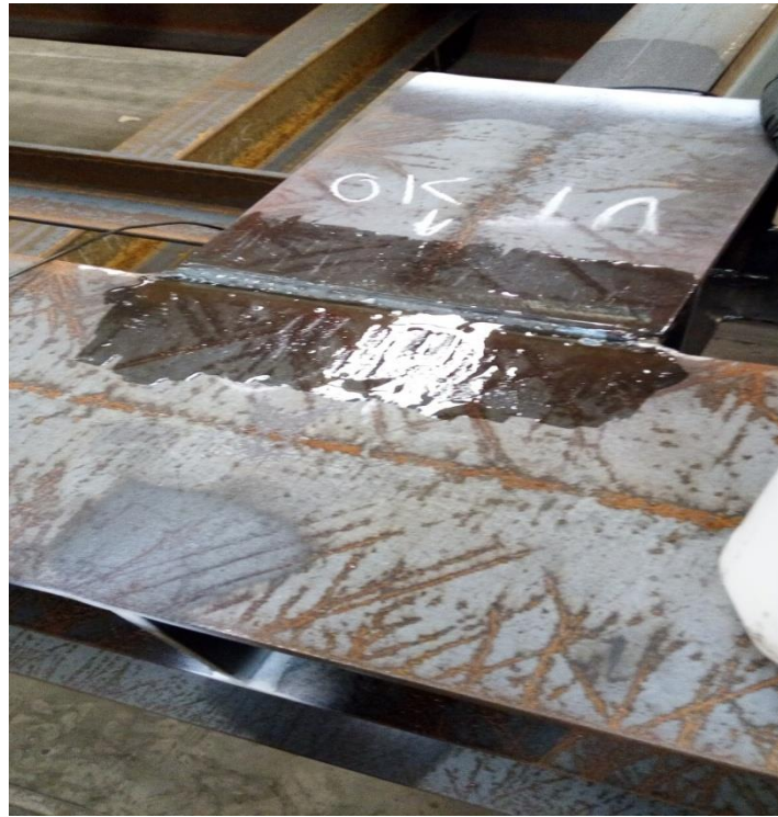
Figure 46: Couplant applied on the weld part (Elctrofer Group, 2017)
