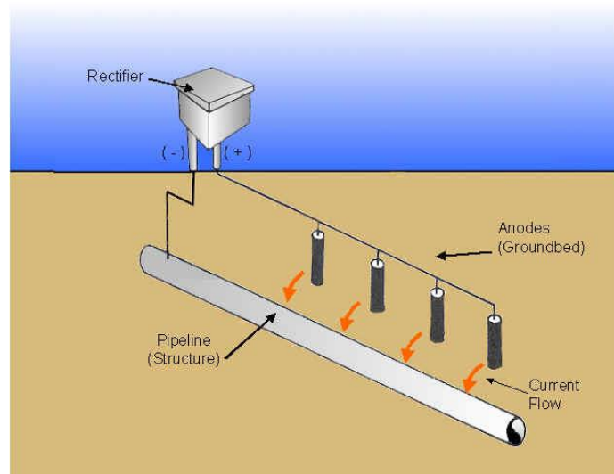
Figure 65: Cathodic protection (Cathodic Protection Systems and Repairs)
