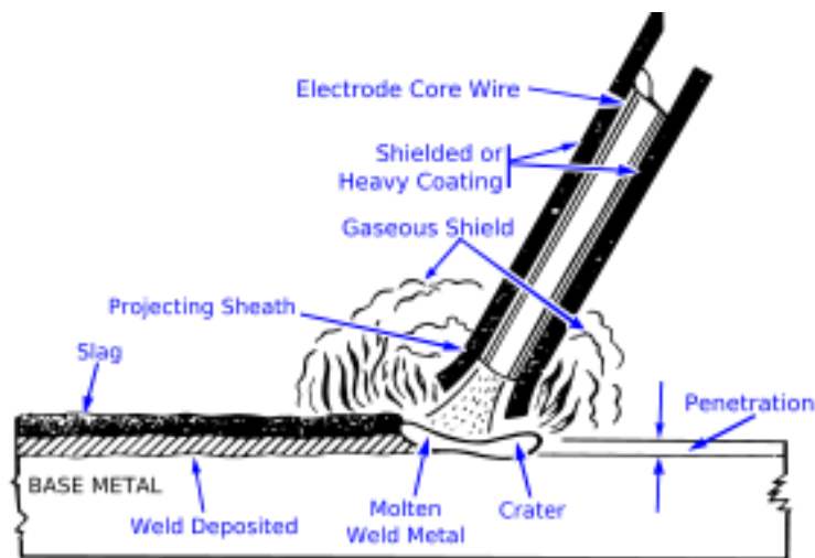
Figure 39: Shielded Metal Arc Welding, process 111(Houldcroft, 1967)
