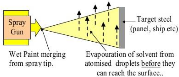
Figure 71: Solvents disappearing from the spray before it reaches the surface (Coating defects)
