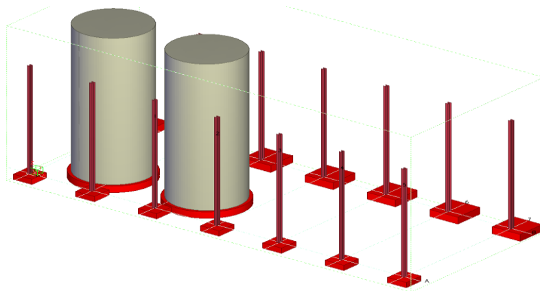
Figure 8: Silos and its structures (Structures, Tekla.)
