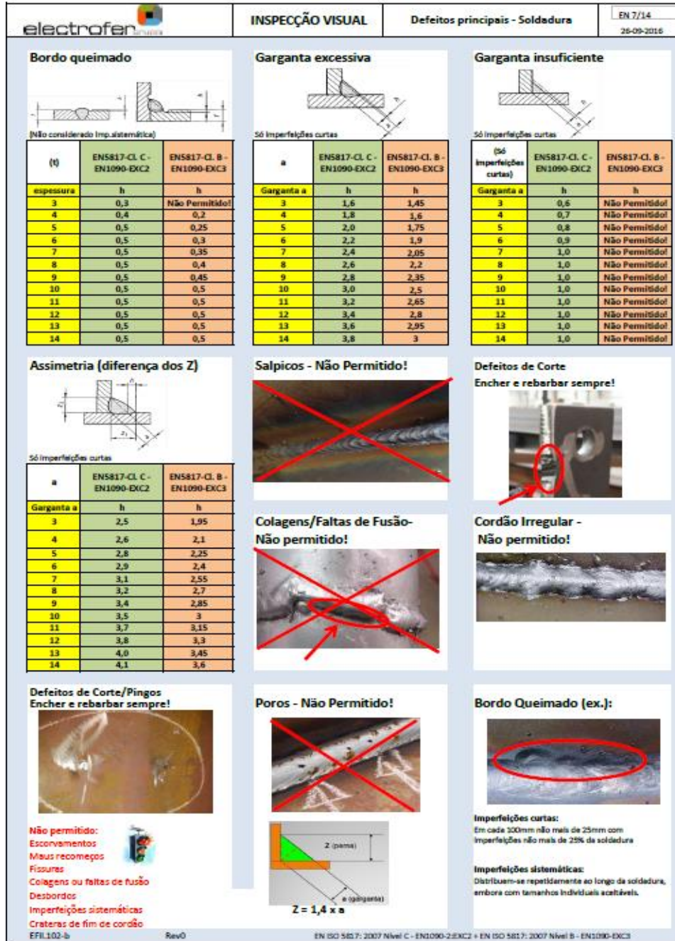
Figure 41: Visual inspection and major welding defects chart (Visual Inspection and Major defects- welding)
