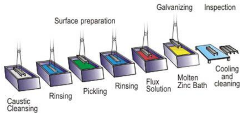
Figure 57: Hot dip galvanizing process (Hot Dipped Wire Galvanizing Line)
