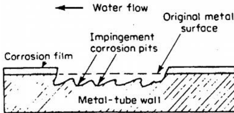
Figure 61: Erosion corrosion in a tube wall (Sharma)
