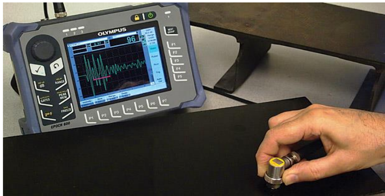
Figure 45: Ultrasonic test equipment (St. Johns group of Institution)
