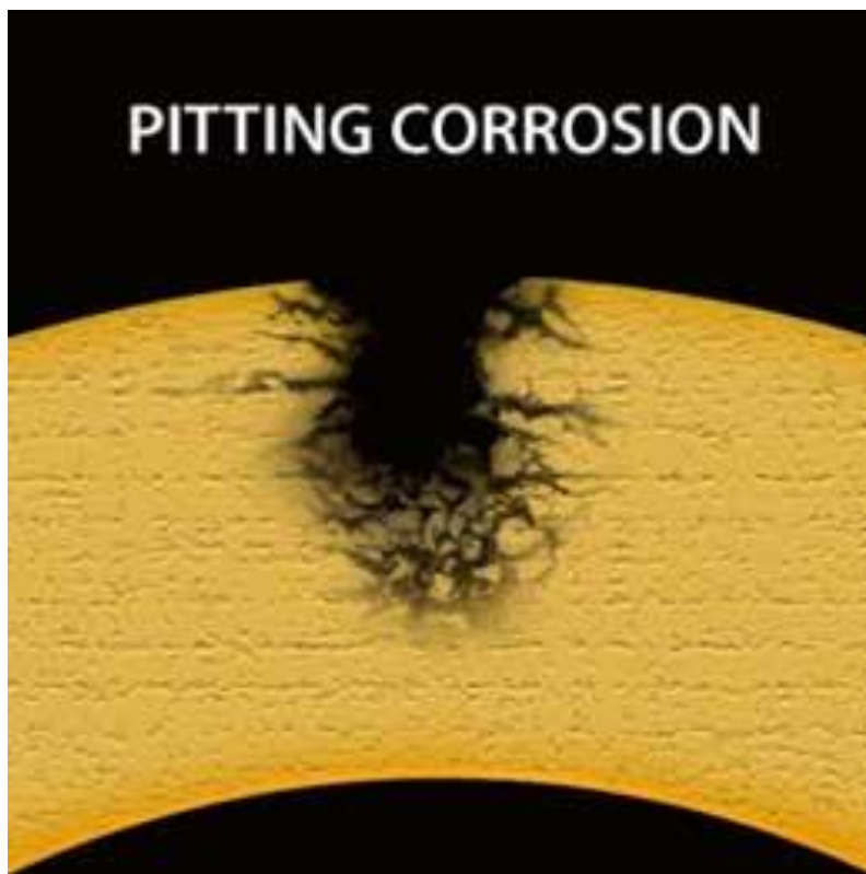
Figure 60: Pitting corrosion (Strategies for Combatting Coil Corrosion, 2010)
