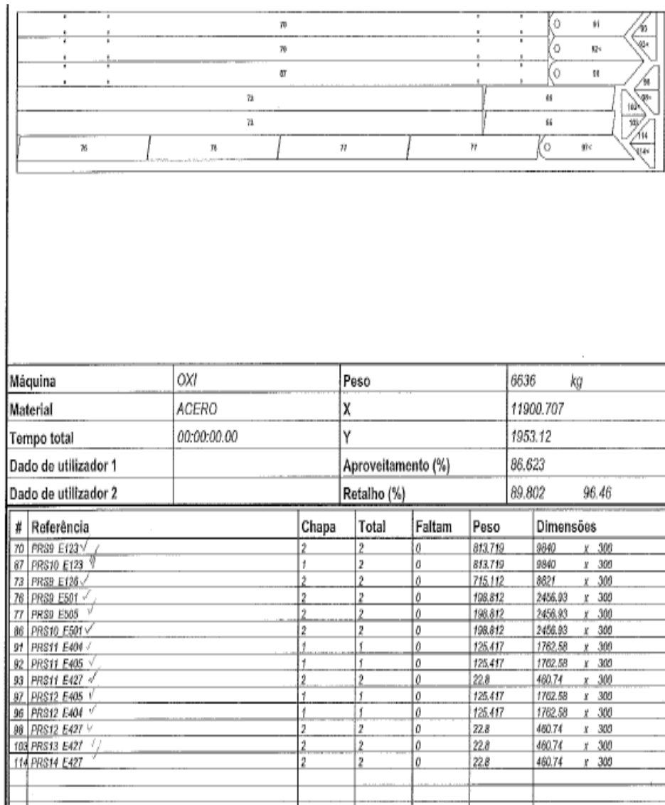
Figure 48: Arrangement of plates for CNC cut (Electrofer Group, 2017)
