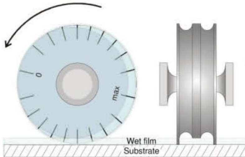
Figure 75: Wheel guage to measure wet film thickness (Using a Wet Film thickness guage)
