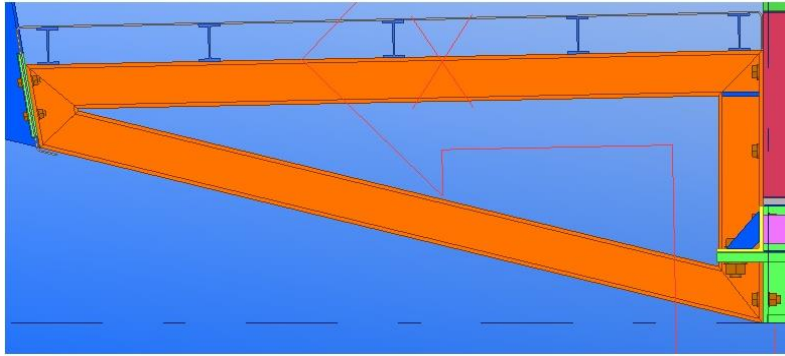
Figure 23: Shoulders for supporting pedestrian's passage (Structures, Tekla.)
