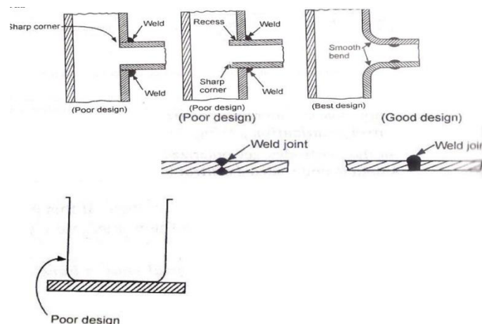
Figure 64: Right angled bends to be eliminated to avoid turbulence which may cause corrosion (Dag Kjernsmo, 2003)
