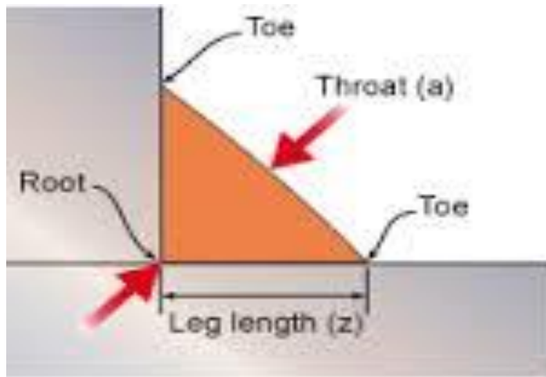
Figure 42: Fillet welding terms (Mathers)
