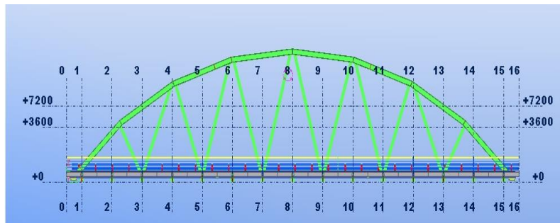
Figure 25: Side view of the arch for bridge (Structures, Tekla.)
