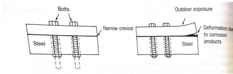
Figure 62: Corrosion products will have volumes higher than steel and cause deformation (Dag Kjernsmo, 2003)
