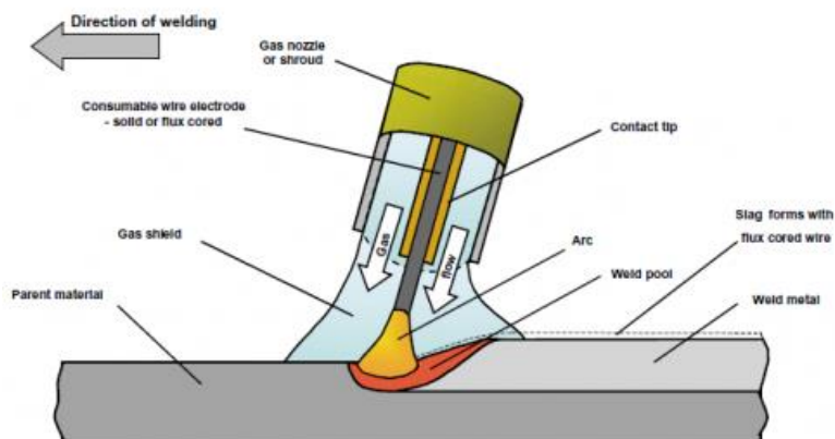
Figure 35: Metal Active Gas welding, process 135 (SteelConstruction.info- The free encyclopedia for UK steel construction information)
