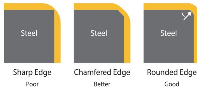
Figure 63: Sharp edges to be rounded to obtain uniform and thick paint coat thickness (Dag Kjernsmo, 2003)
