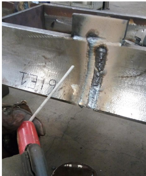
Figure 56: Shielded metal arc welding process (Elctrofer Group, 2017)
