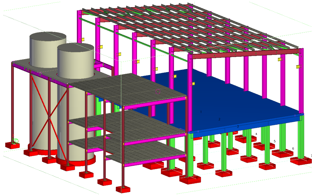
Figure 14: The completed model of silos and its structures (Structures, Tekla.)
