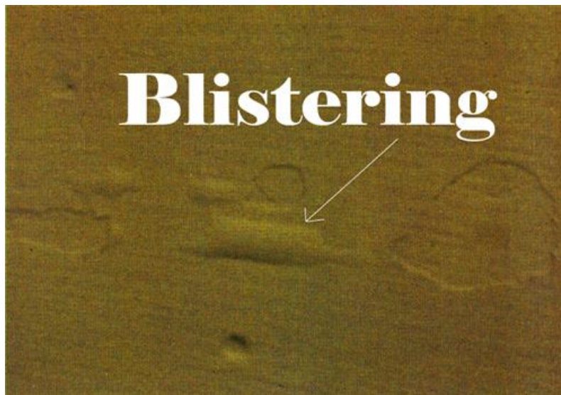
Figure 68: Blistering due to entrapped air or solvents in the coating (Davi PAints, 2009)
