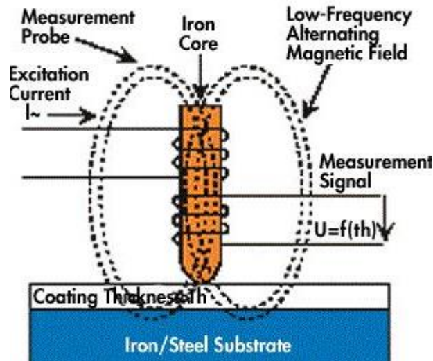
Figure 76: Magnetic induction instrument (Magnetic Induction Process)
