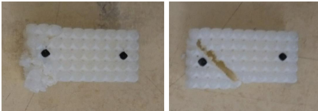
Figure 3: Different failure modes of specimens of the same type during mechanical testing.
