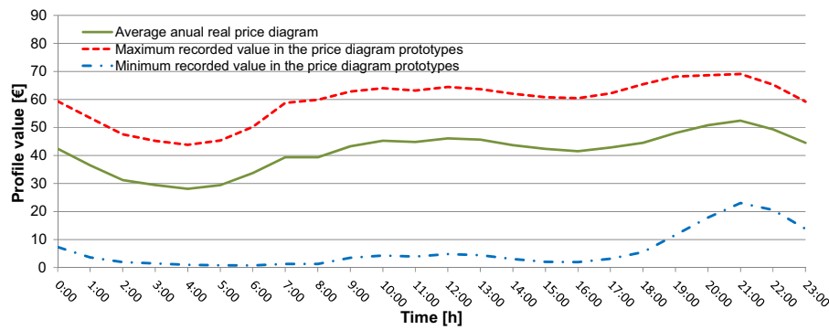
Fig. 14. Prototypes price range variation, from October 2012 to September 2013.
