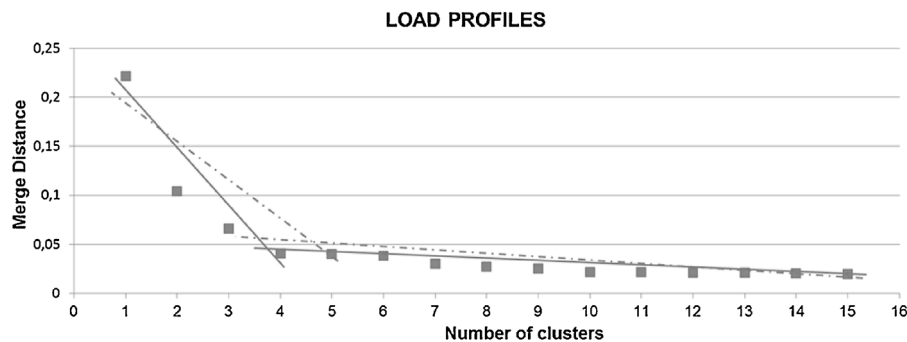
Fig. 4. Relation between the selected number of clusters and the merge distance for the case of load demand.
