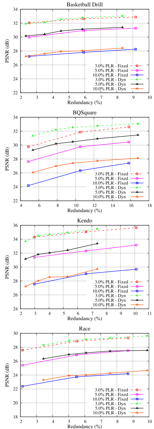
Fig. 9. Decoded video quality for different amounts of redundancy, selected using a fixed approach and the proposed method.
