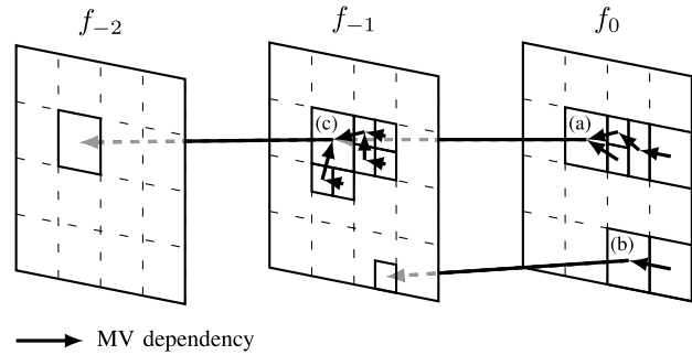
Fig. 5. Example of temporal and spatial MV dependencies in HEVC.
