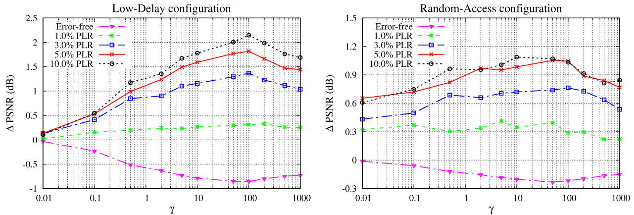
Fig. 8. Influence of the \gamma parameter in the average quality gains, comparing with Ref , for different packet loss ratios.
