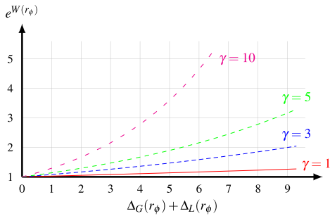
Fig. 4. Exponential weight as a function of the global and local deviations.
