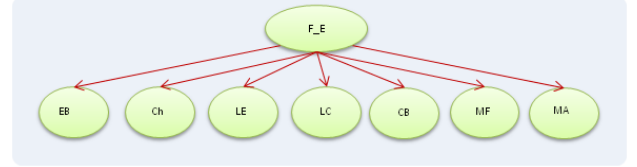
Figure 4. Bayesian Network to classify facial expression – approach 2.
