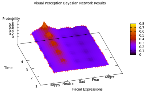
Figure 5. Classifying facial expressions: approach 1 results.
