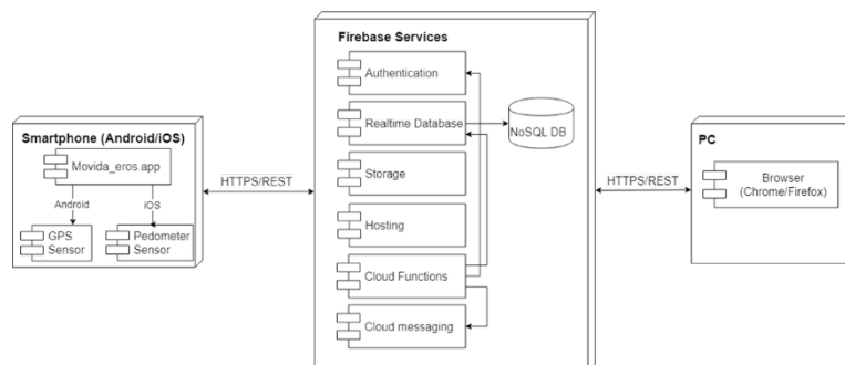
Fig. 1. MOVIDA.eros architecture
