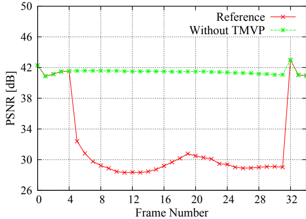
Fig. 2: Error propagation for the Book Arrival sequence encoded at 2Mbps (Frame #4 is lost).
