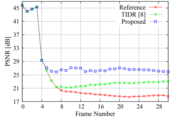
Fig. 4: Quality obtained with the different approaches tested in the HEVC when the Frame #4 is missing for the BQSquare sequence @ 1.0 Mbps.
