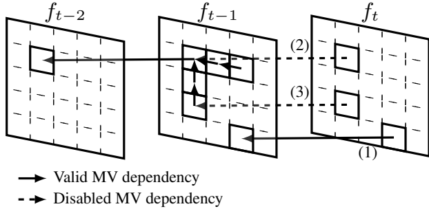
Fig. 3: Proposed approach to use the temporal motion vector candidate in the HEVC encoder.
