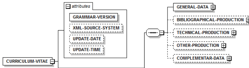
Figure 3. DeGóis® CV XML Schema
