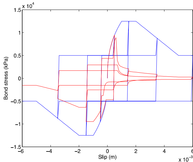
Fig. 4 – Qualitative comparison between the implemented bond stress-slip model without (blue) and with (red) the effects of yielding and cyclic degradation
