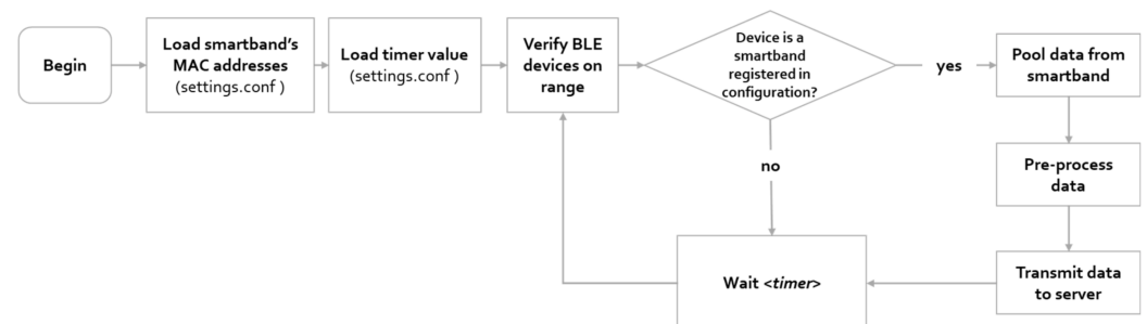
Figure 10. Operation algorithm of the gateway script.
