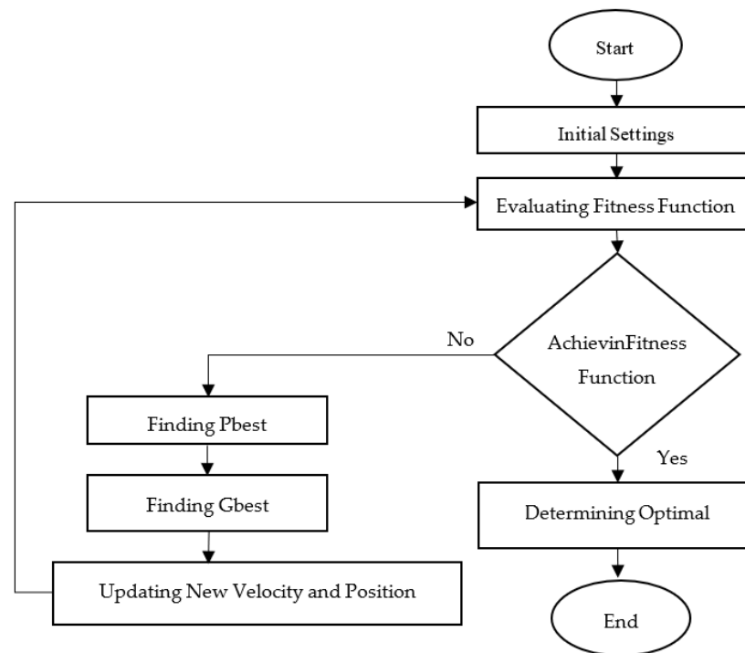
Figure 4. PSO flowchart.
