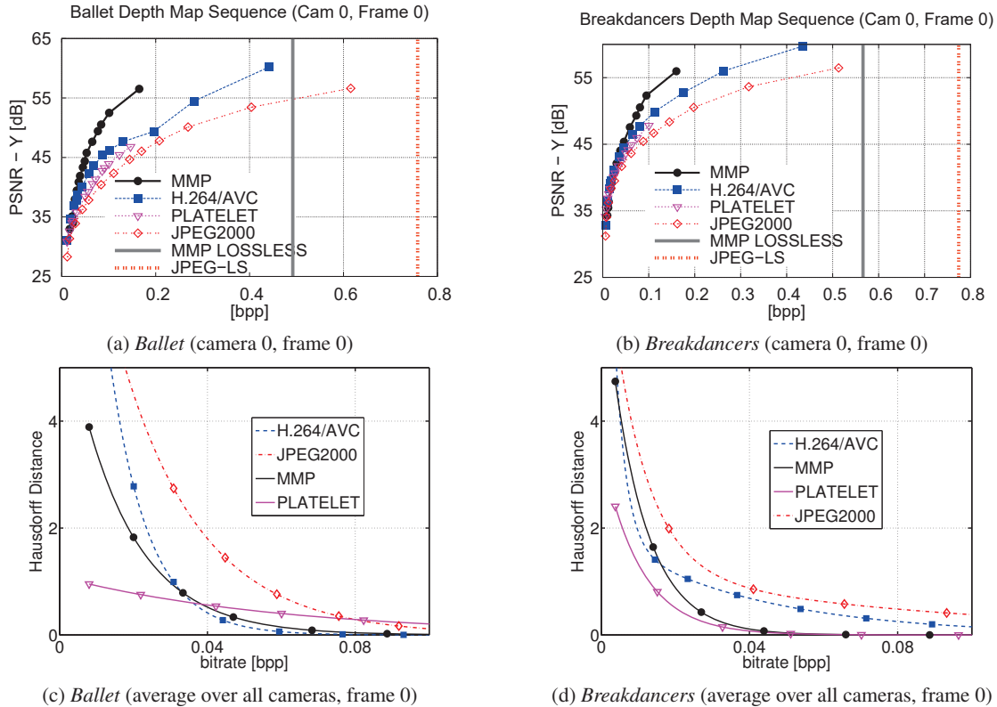
Fig. 1. R-D curves and Symmetrical Hausdorff distance for depth map coding.
