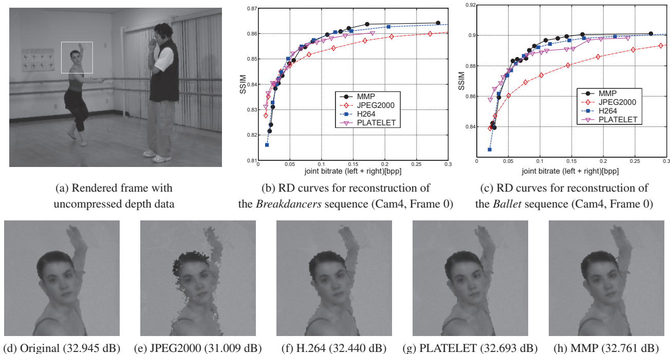
Fig. 2. Reconstruction of the first frame of the 4th camera of Ballet sequence, using the original views of the 3rd and 5th cameras and respective encoded depth maps. Figures (e)-(h) show details of the reconstruction with each depth map encoded at 0.075bpp.
