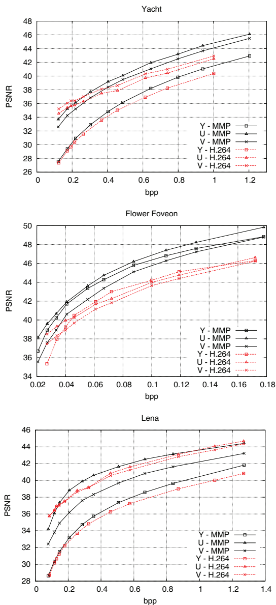
Fig. 3: RD results for MMP using the proposed method and H.264/AVC for YUV images.
