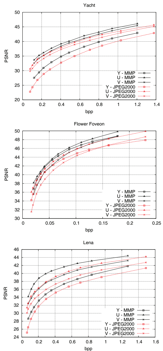
Fig. 4: RD results for MMP using the proposed method and JPEG2000 for YUV images.
