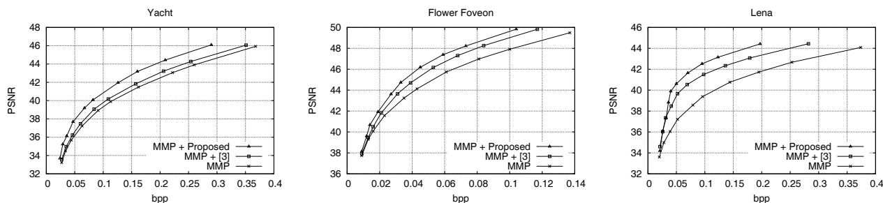
Fig. 1: Compression of the U chroma using MMP, MMP and the proposed algorithm and MMP with the method in [3].
